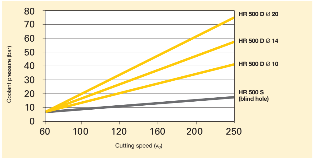
Coolant pressure - cutting speed valid for standard dimensions. Preconditions: sufficient capacity of coolant pump
