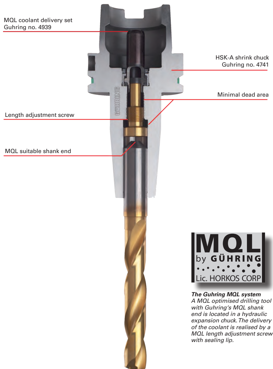
Shank end suitable for minimal quantity lubrication without build-up or dead pockets of coolant.
